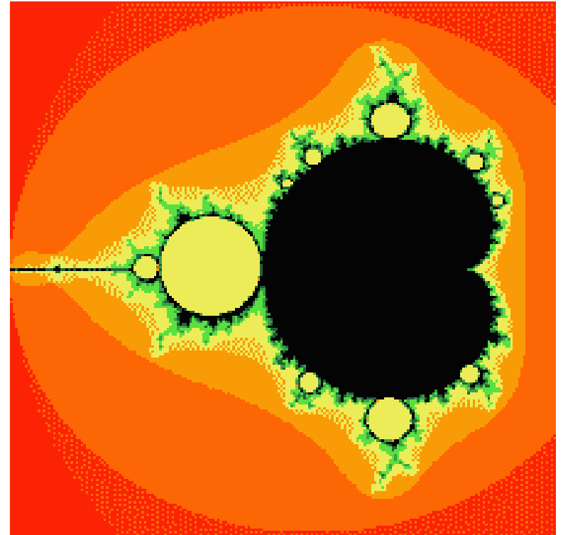
Mandelbrot Set
